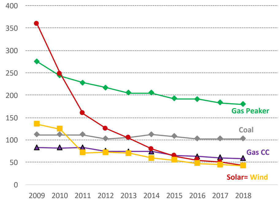
Mean Levelized Cost of Electricity ($/MWh)
